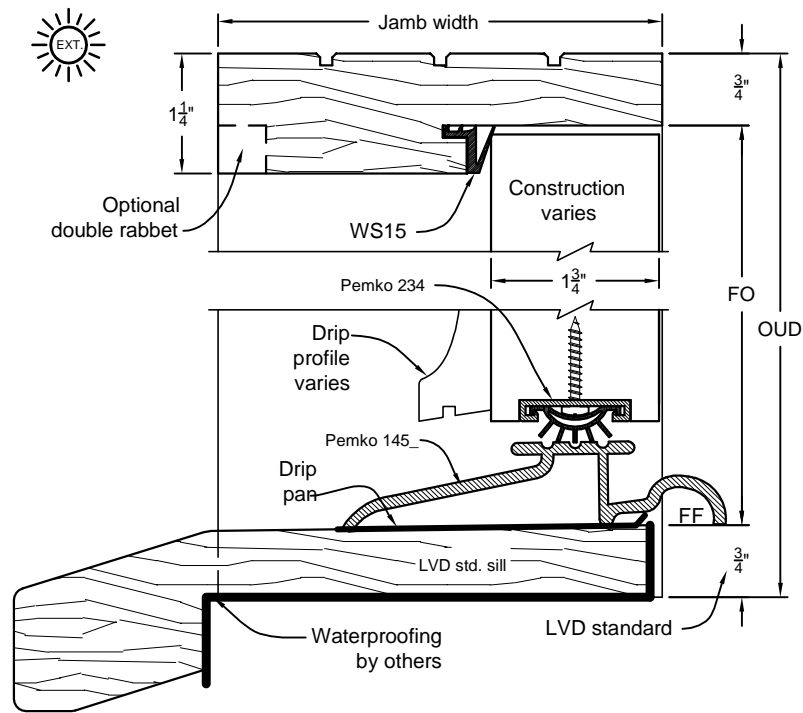
TYP. HEAD & SILL DETAIL SECTION 1-3/4" EXT. INSWING DOOR
