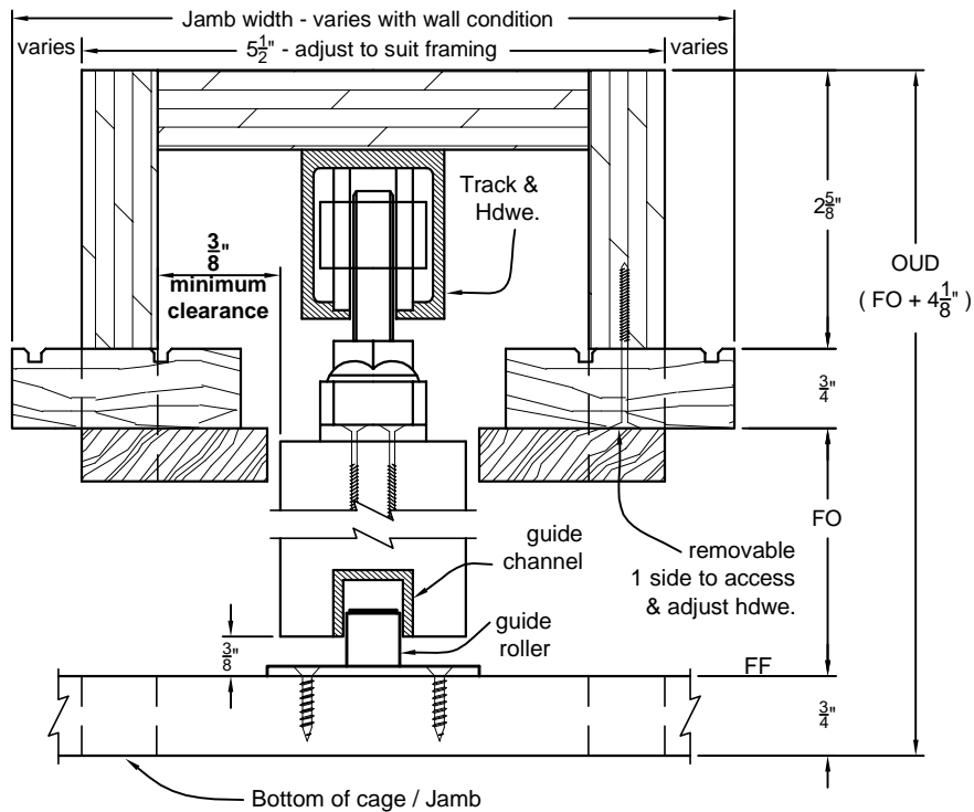
TYP. HEAD & SILL DETAIL SECTION POCKET DOOR - 5-1/2" CAGE w/STOPS
