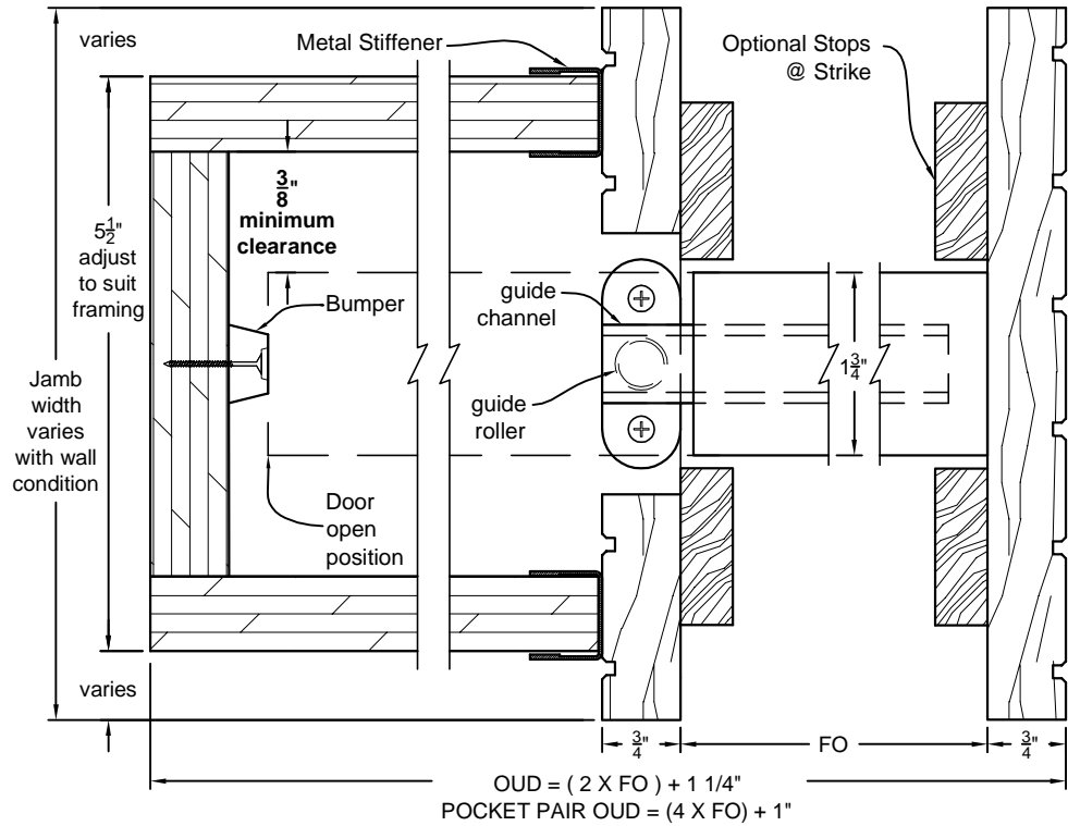
TYP. JAMB DETAIL SECTION POCKET DOOR - 5-1/2" CAGE w/STOPS
