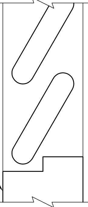
LOUVER DETAIL @ TOP & BOTTOM RAIL 1 3/8" LOUVER DOOR
